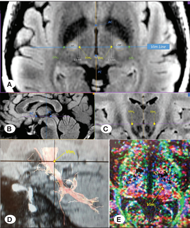
Figure 2: VIM point determination in MRI (T2 flair sequences) using the VIM line technique. A) axial; B) sagittal; C) coronal; D) dentatorubrothalamic track in diffusion tensor imaging (DTI)/diffusion-weighted imaging (DWI) sequence; E) region of interest (ROI) placement in DTI sequence. AC: anterior commissure, PC: posterior commissure, CST: cerebrospinal track, GPe_L : left external globus pallidus, GPe_R : right external globus pallidus, VIM_L : left ventral intermediate nucleus of the thalamus, VIM_R : right ventral intermediate nucleus of the thalamus.
